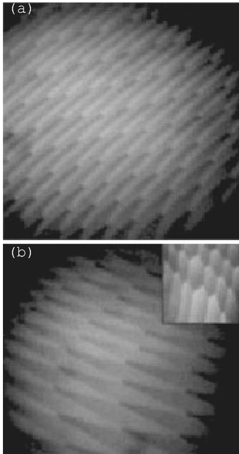
FIG. 4. (a) Brick wall texture in a 50.6 film at 52 °C. (b) Elongated hexagonal texture at about 51.8 °C. The inset shows a honeycomb texture at about 51.5 °C. The horizontal dimensions are about 250 \mu\text{m} for (a), 200 \mu\text{m} for (b), and 100 \mu\text{m} for the inset in (b).
