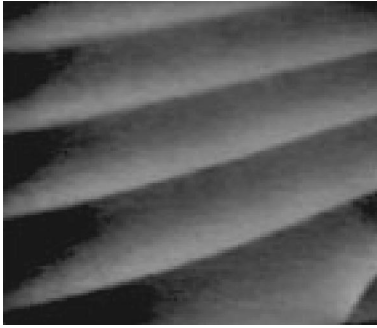
FIG. 2. Line texture (splay texture) in a 50.6 film at 50.8 °C showing typical modulated sharp lines separating bands with continuously changing intensity. The horizontal dimension is about 150 \mu\text{m} .
