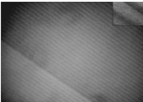
FIG. 3. Stripe texture in a 50.6 film at 54 °C, showing alternating light and dark uniform bands of unequal widths. The horizontal dimension is about 200 \mu\text{m} . The inset shows details of the adjacent light and dark stripes.
