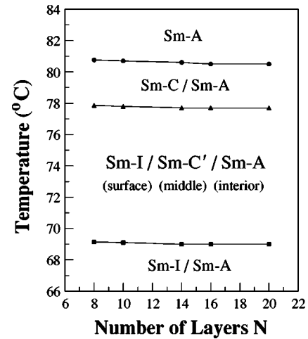
FIG. 6. Phase diagram for 70.7 with Sm-I/Sm-C'/Sm-A denoting the coexistence, as a function of distance from the surface, of three distinct phases: an outermost Sm-I layer, several layers of a middle Sm-C' phase, and a Sm-A interior [13].
