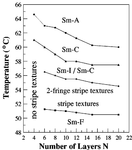
FIG. 5. Optical phase diagram for 50.6.
